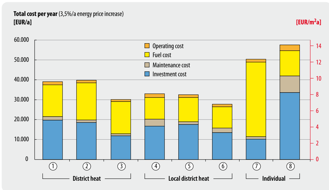
Figure 8: Total annual cost of heat supply of a passive house neighbourhood comprising 34 dwellings with a floor space of 120 m 2 each (calculation to VDI 2067, energy price increase of 3.5% p.a.).
