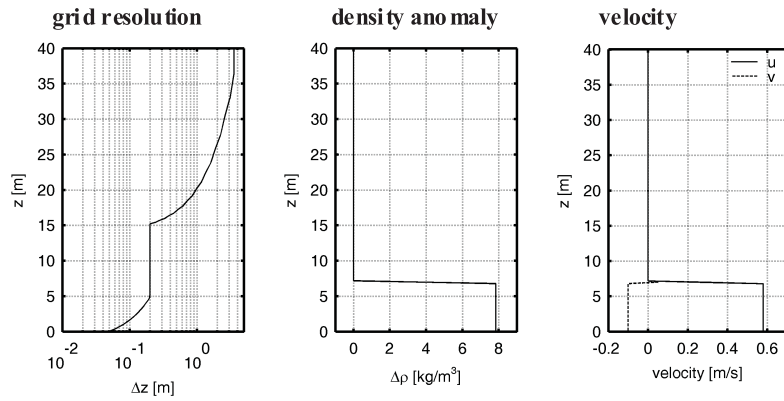
Figure 3.62: Grid resolution and initial conditions for the one-dimensional simulations of entrainment in an undisturbed gravity current.
