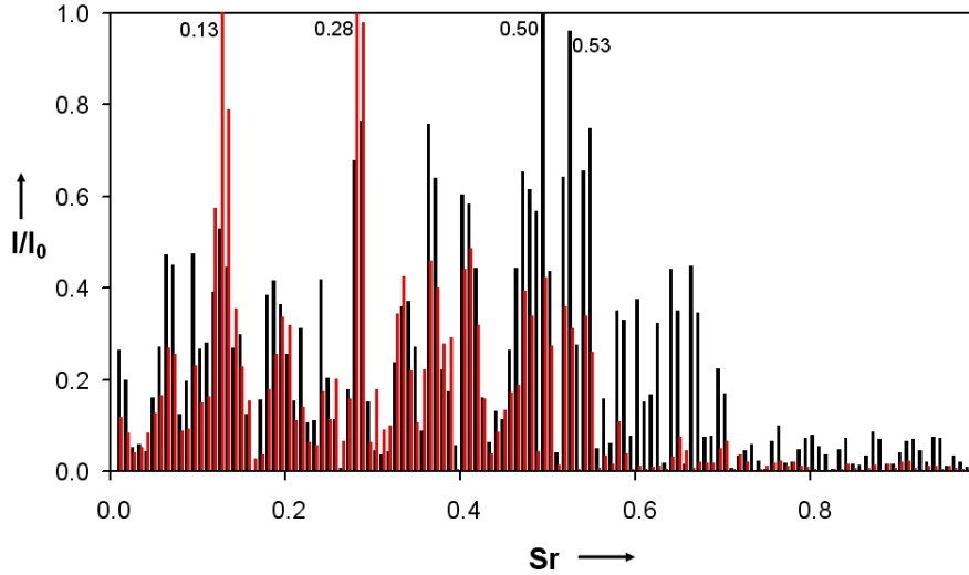
Figure 3.25: Normalised Strouhal-spectrum.
