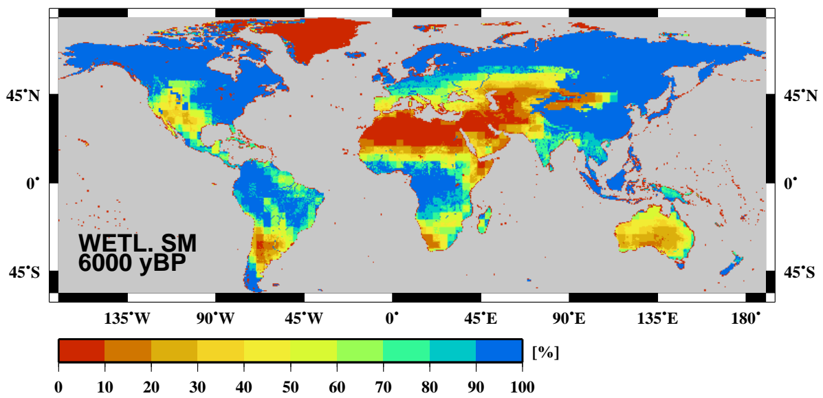
Figure B.7.: Relative soil moisture saturation for wetlands in the Mid Holocene simulation.
