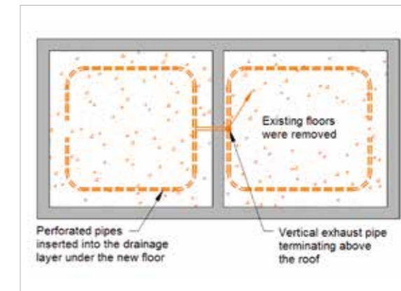
Fig. 7. Network of perforated pipes in the drainage layer suitable for remediation
