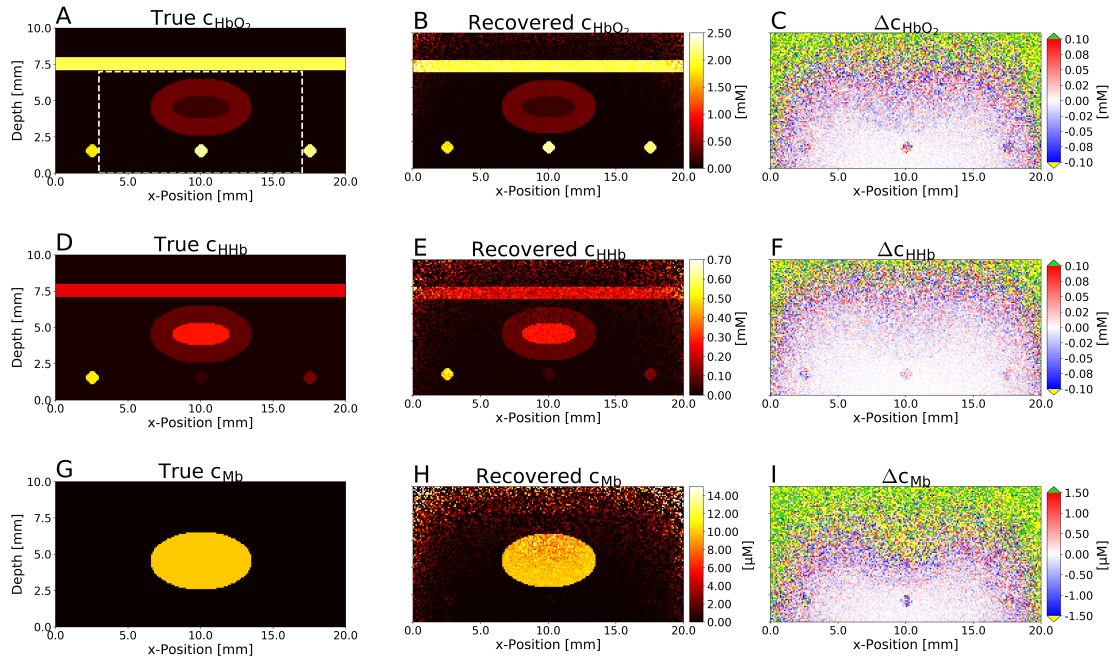
Fig 4 2D cross-sectional xz -images of the true and recovered chromophore concentrations together with the absolute error at y = 10 mm. Left column: True chromophore concentrations. Center column: recovered concentrations. Left and center column share the same colorbar. Right column: absolute concentration error. Voxels where the error exceeds the limits of the colorscale are rendered in green and yellow. In A, the reduced background subvolume 1* is illustrated as a white dashed rectangle. Because background voxels far away from the source exhibit large errors due to low SNR, this reduced subvolume is used for calculation of average concentrations.
