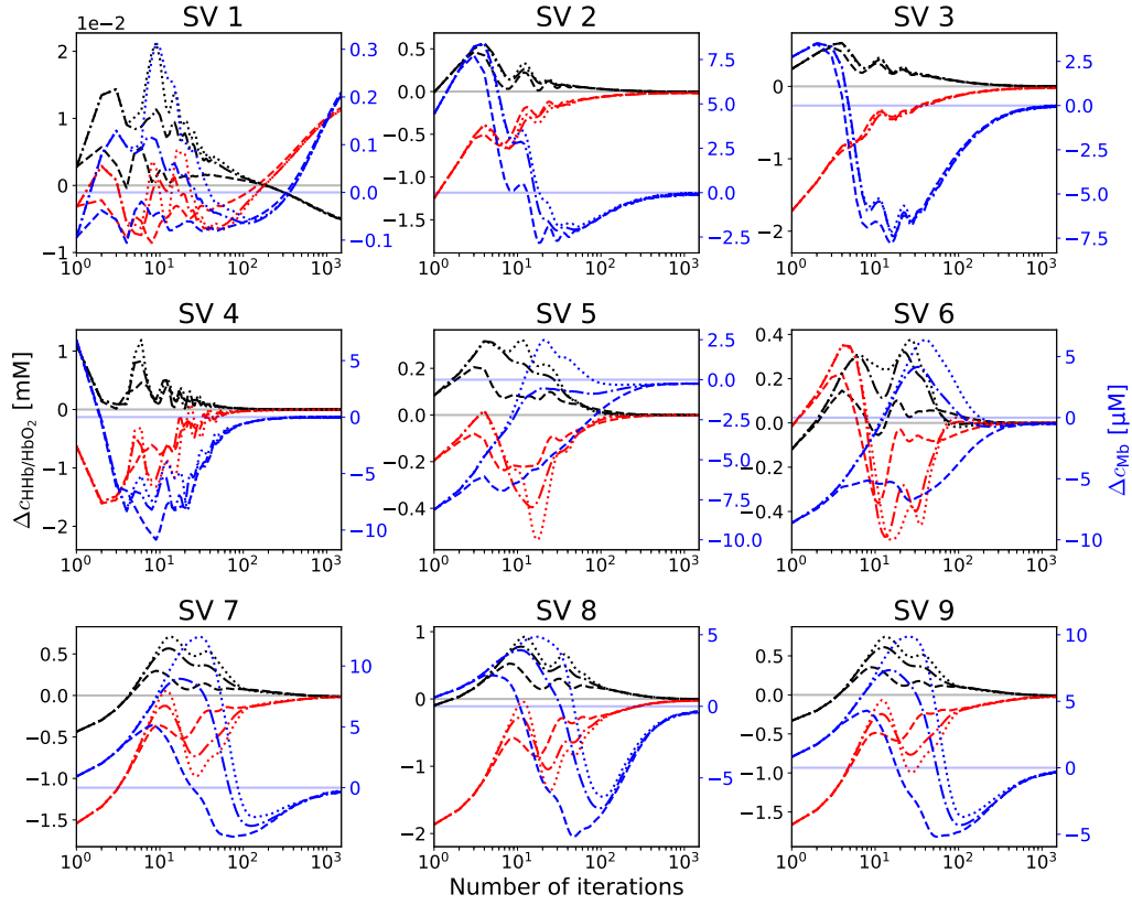
Fig 7 Convergence of the true and recovered concentrations for inversions incorporating the gradient term of the adjoint radiance for N_L = 4 (dotted line, \cdots ), N_L = 0 (dashed-dotted line, - \cdot - ), and without the adjoint term (dashed line, -- ). The chromophores are shown in blue (Mb), red ( \text{HbO}_2 ) and black (Hb). Horizontal lines in light color depict perfect convergence, i.e. \Delta c = 0 .
