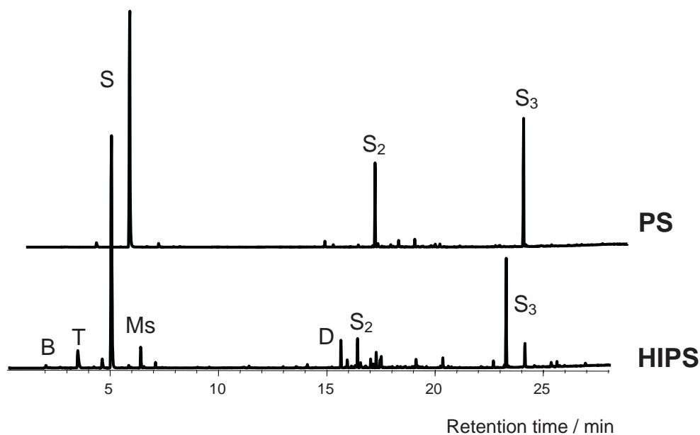
Figure 1. Pyrolysis products of PS and HIPS at 500°C. B, butadiene; T, toluene; S, styrene; Ms, \alpha -methylstyrene; D, 1,3-diphenylpropane; S 2 , styrene dimer; S 3 , styrene trimer.
