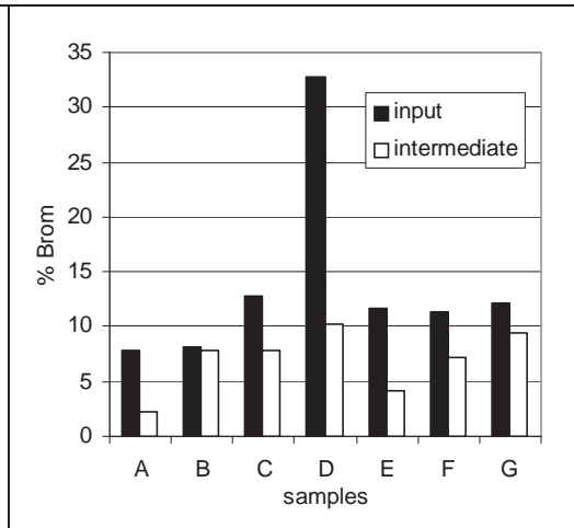
Fig 11: Bromine reduction obtained during the Fraunhofer-IVV recycling process.
