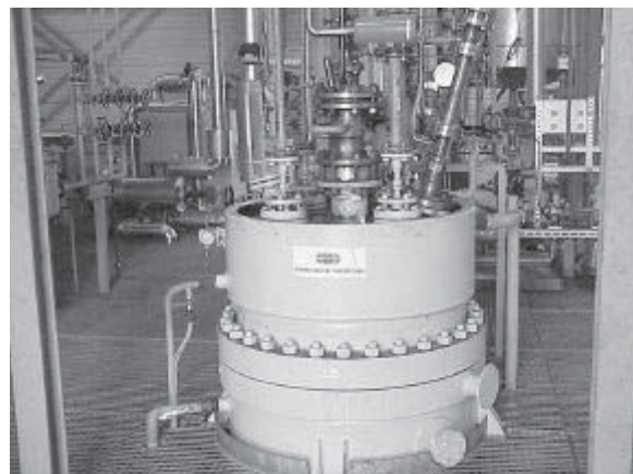
Fig. 15: Top of the 5+ MW(th) pilot scale pressurised entrained flow gasifier at Babcock Borsig Power (BBP), Freiberg, Saxony.
