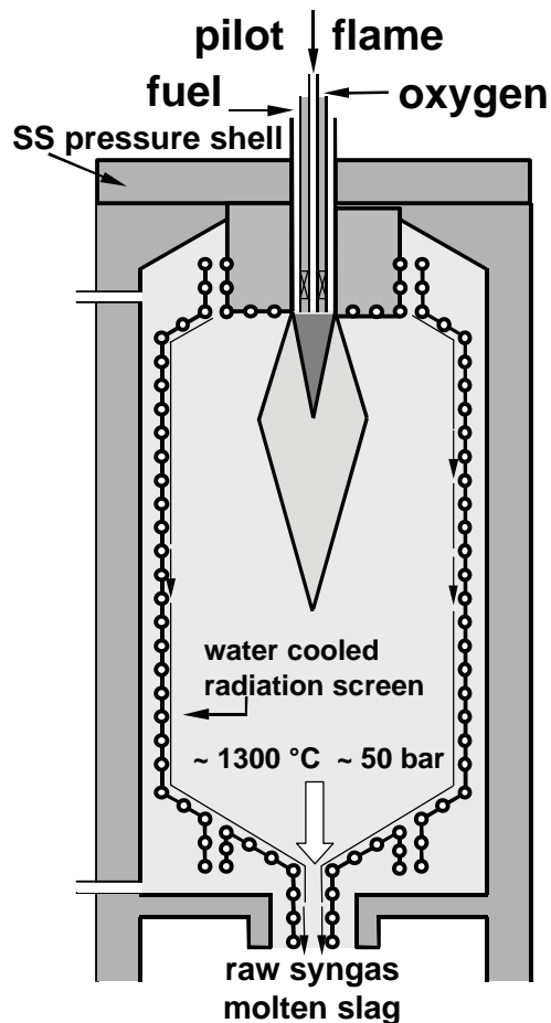
Fig. 14: Slugging entrained flow gasifier for operation at high temperature and pressure. The characteristic radiation screen with SiC-liner, is cooled with pressurised water, to keep the pressure resistant steel shell at low temperatures.
