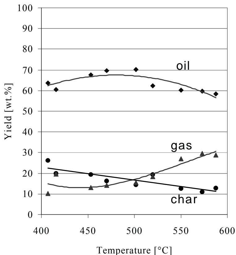
Fig. 2 Typical yields of fast pyrolysis experiments with the pilot plant
