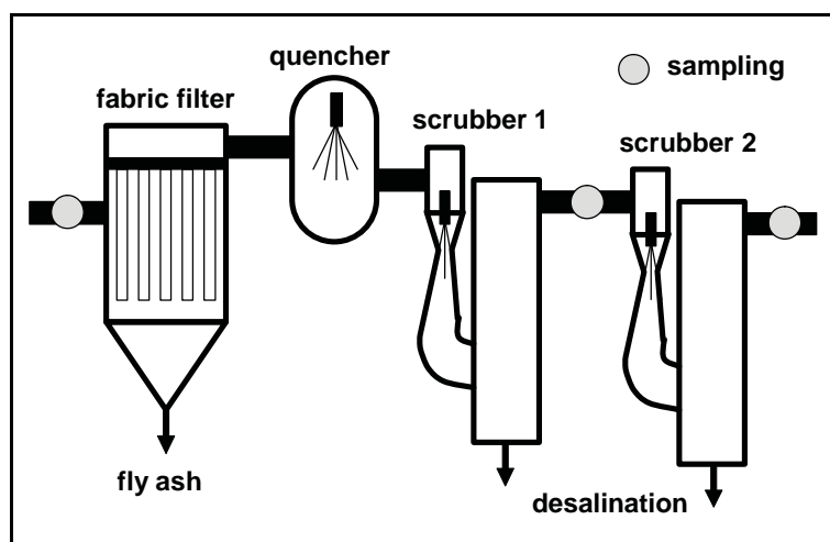
Fig. 2 Scheme of part of the TAMARA air pollution control system with sampling points
