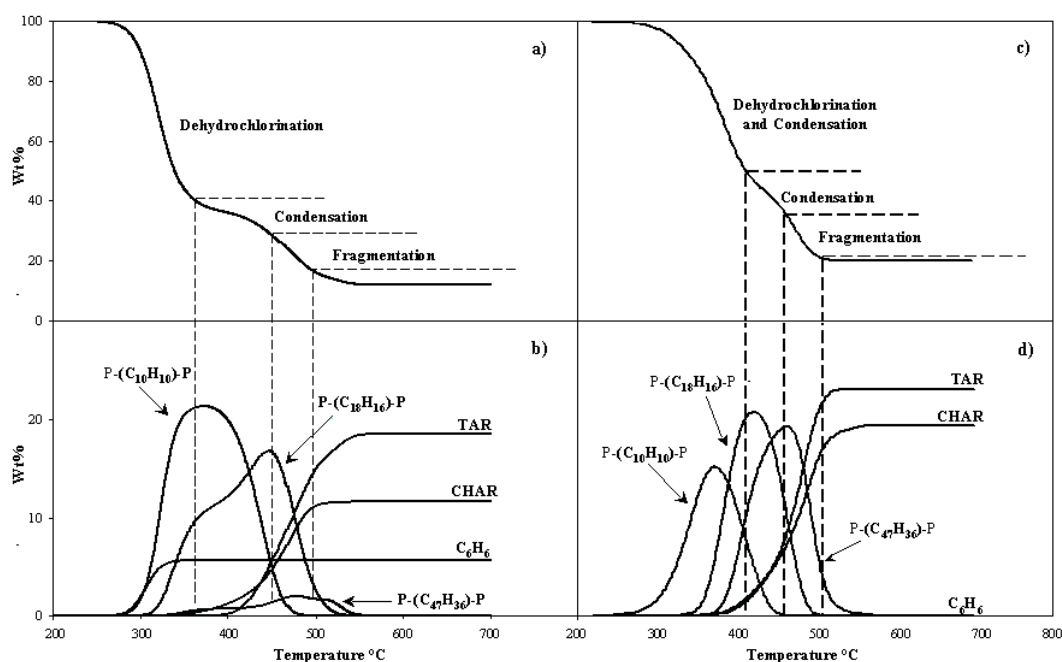
Figure 2. Predicted dynamic TGA with an heating rate of 10°C/min:
