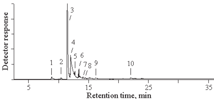
Fig. 9. Treatment of 2,4-dichlorophenol in a closed ampoule with polypropylene under an inert atmosphere at 500 °C for 20 min
