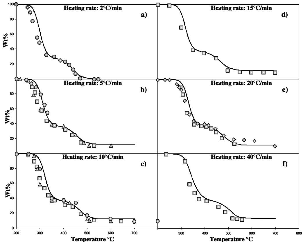
Figure 7 Dynamic TGA of PVC at different heating rates, predicted data are reported with line, experimental data with marks:
