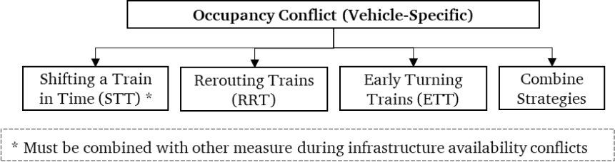
Figure 6.5 Elemental conflict solution alternatives for occupancy and infrastructure availability conflicts (by author)
