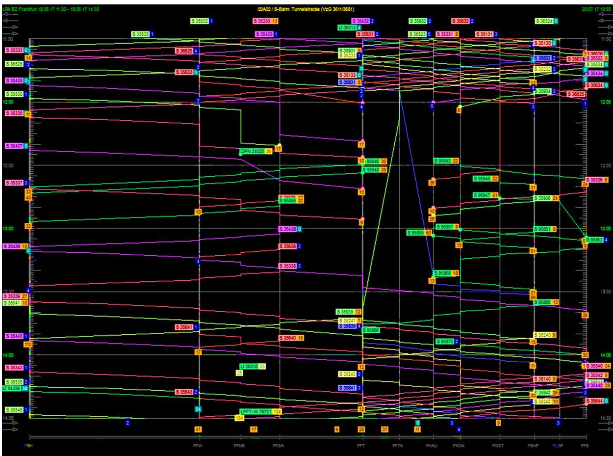
Figure 14.2 Traffic diagram depicting the handling of a disruption with a total blockage in the tunnel area of the S-Bahn Rhein-Main network (DB Regio AG 2017)
